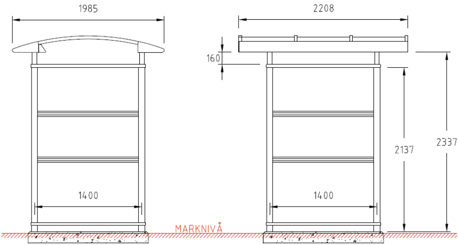
1301012 City 90 for parkeringsautomat Micro 2208 x 1985 mm
