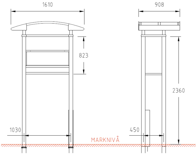
1301047 City 90 for parkeringsautomat Ticket 908 x 1610 mm
