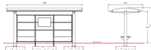
1301057 City 90 Piazza P (1 felt) 5788 x 2645 mm
