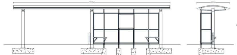
1301053 City 90 Piazza R (2 felt) 10764 x 2235 mm
