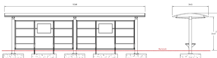
1301058 City 90 Piazza P (2 felt) 10268 x 2645 mm
