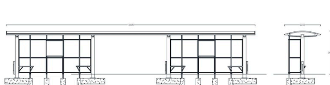
1301054 City 90 Piazza R (3 felt) 15490 x 2235 mm
