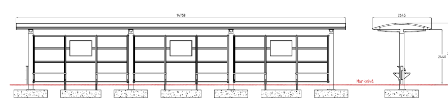
1301059 City 90 Piazza P (3 felt) 14758 x 2645 mm
