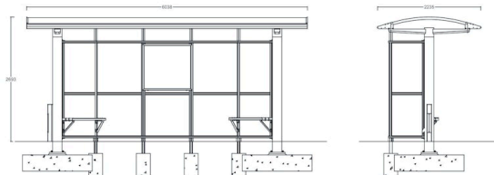
1301052 City 90 Piazza R (1 felt) 6038 x 2235 mm
