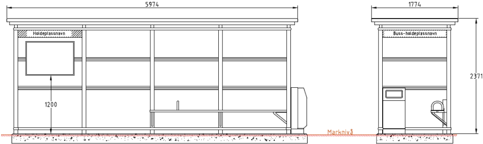
4101003 Edgy (4 felt) 5974 x 1774 mm
