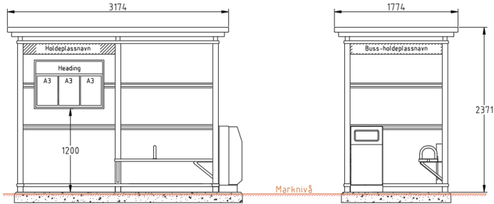
4101001 Edgy (2 felt) 3174 x 1774 mm
