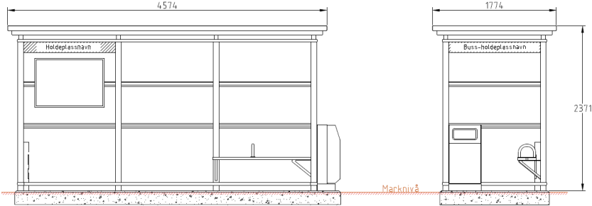
4101002 Edgy (3 felt) 4574 x 1774 mm
