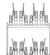
Bike-Up Basic Twin Tower 4+4+4+4
